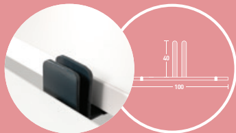
BENCH BRACKET
