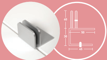
STANDARD CLAMP BRACKET - 30MM
